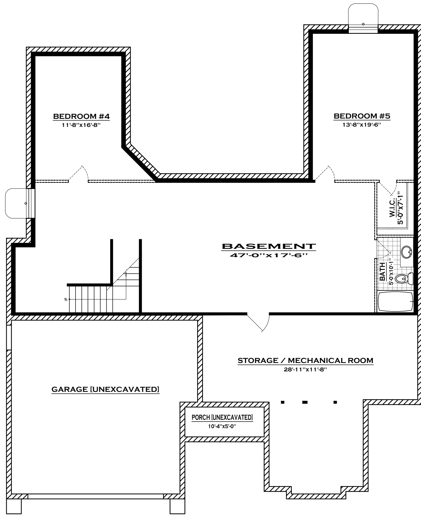
BASEMENT PLAN 2,159 SQ. FT.
