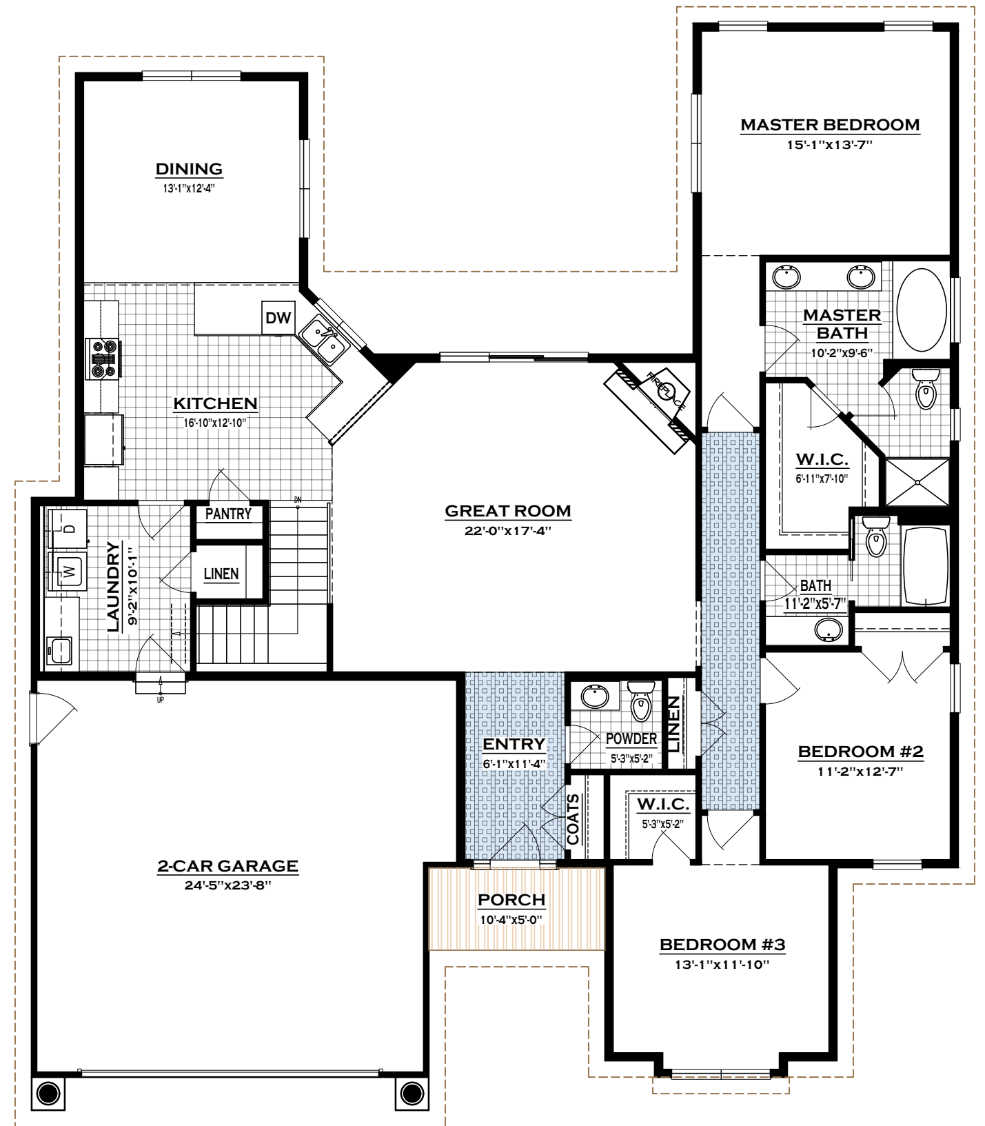
GROUND FLOOR PLAN 2,159 SQ. FT.
