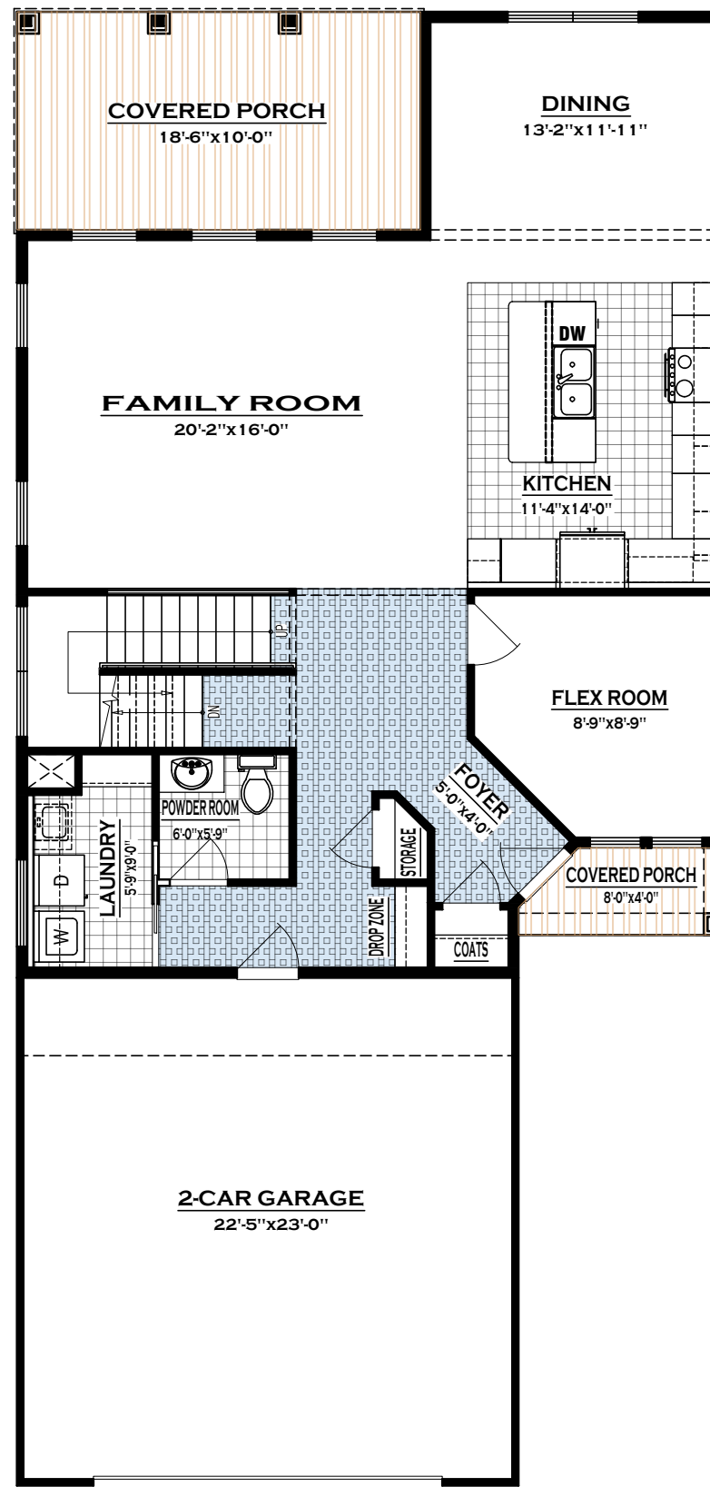
FIRST FLOOR PLAN 1,202 SQ. FT.
