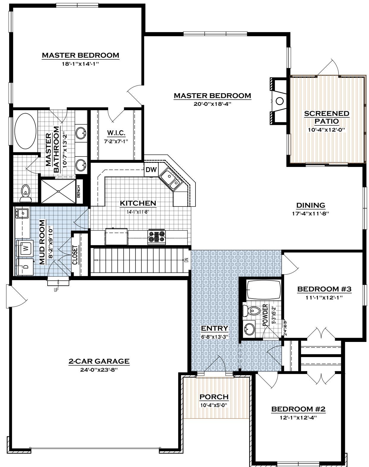
GROUND FLOOR PLAN 2,098 SQ. FT.
