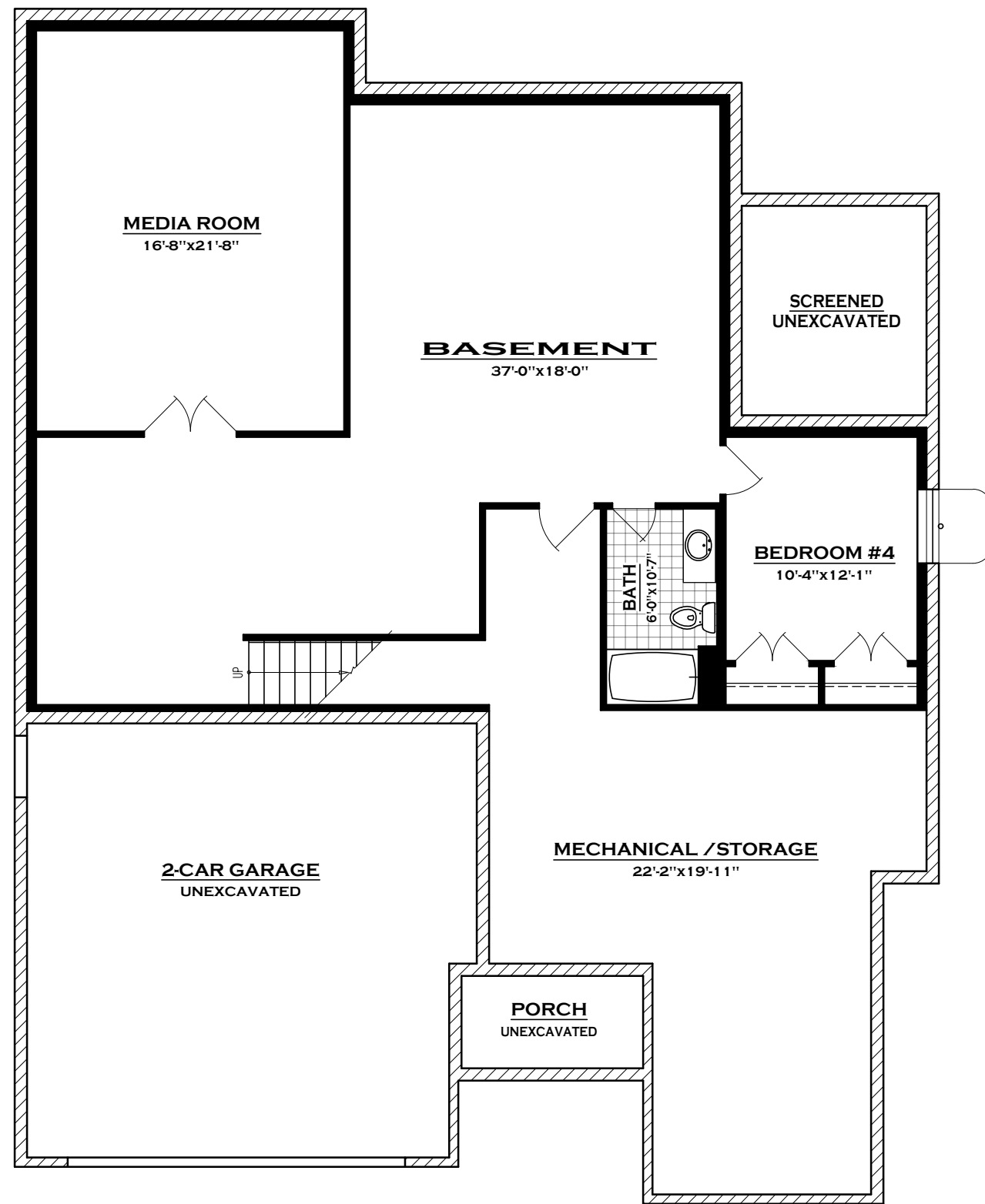
BASEMENT PLAN 2,098 SQ. FT.
