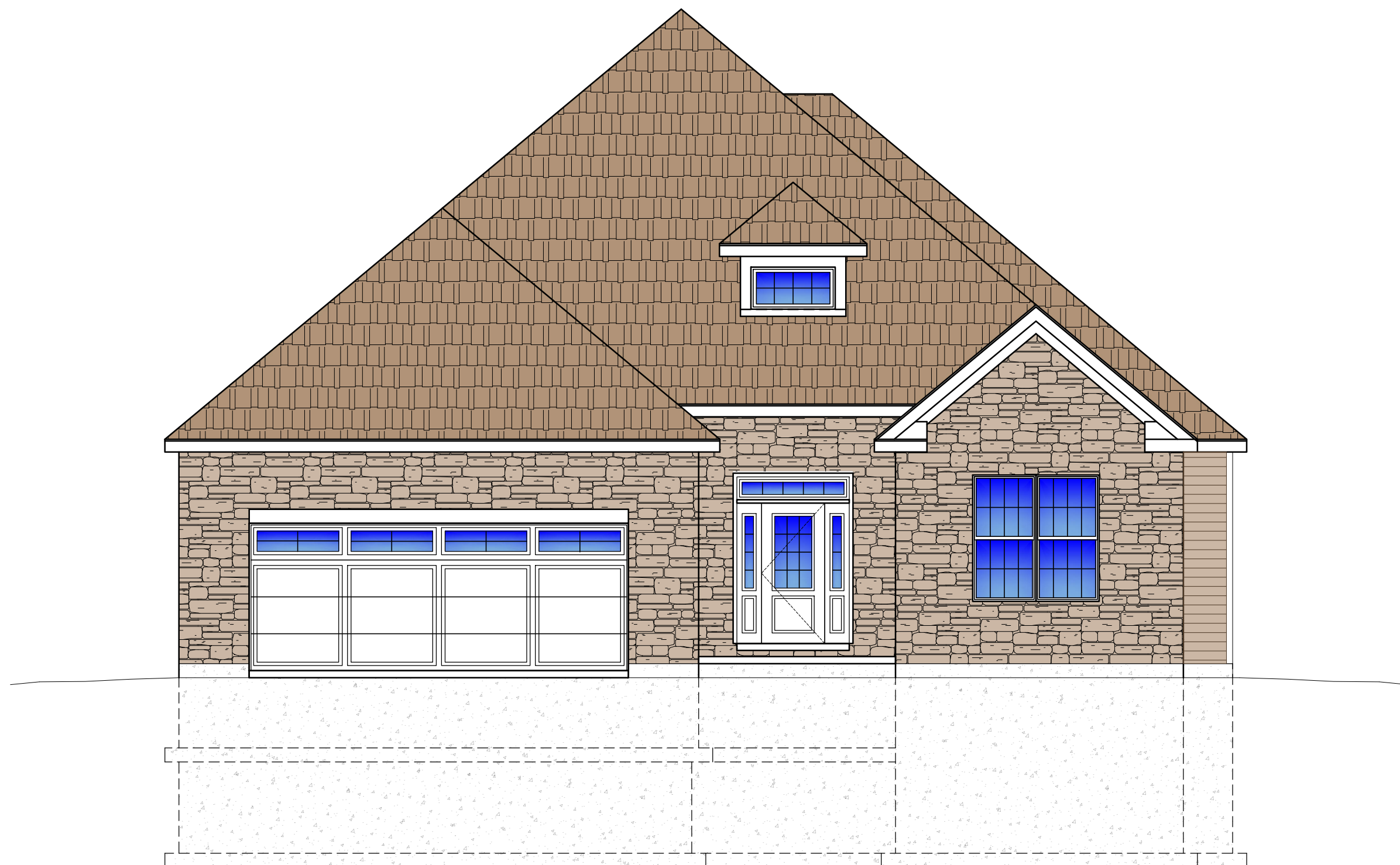
FRONT ELEVATION
