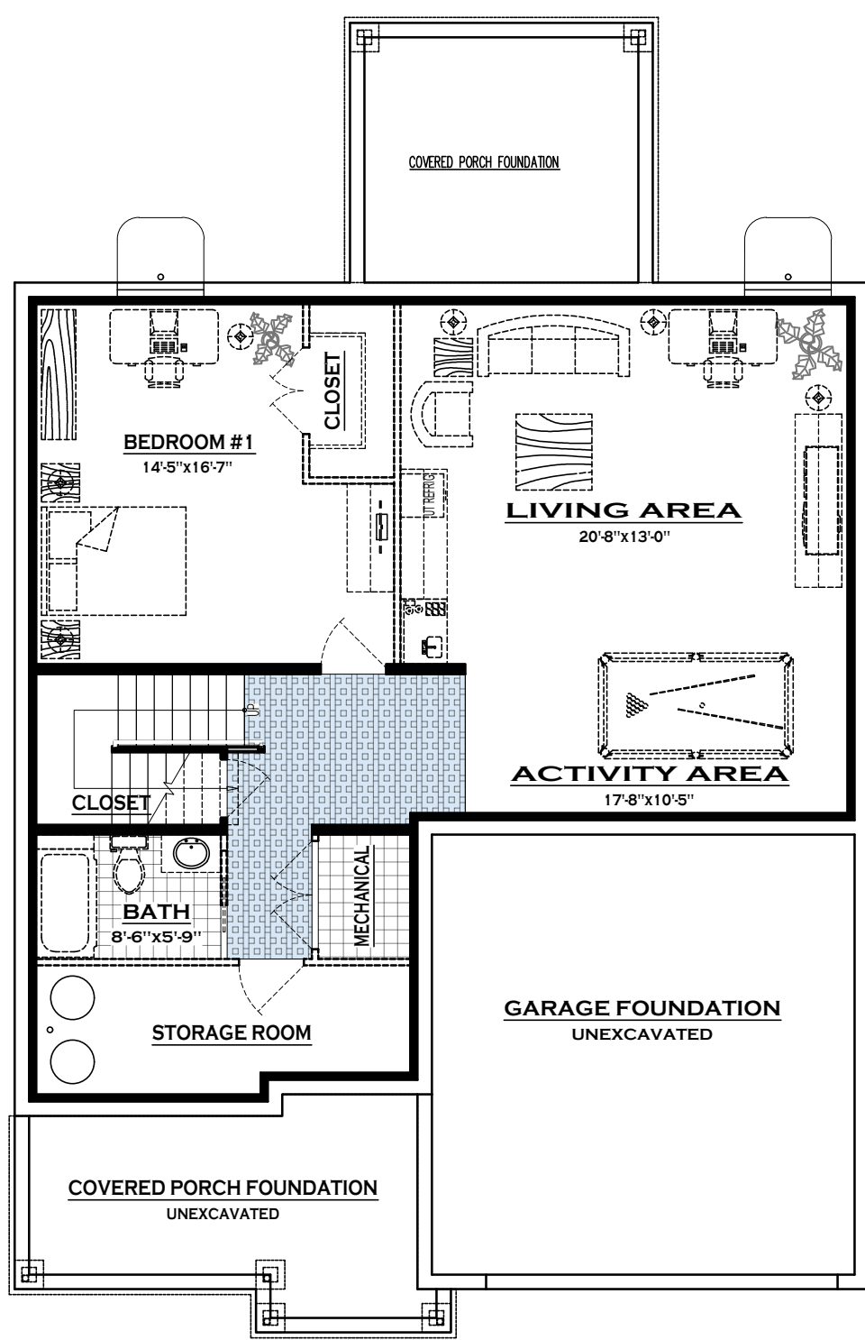
BASEMENT PLAN 1,251 SQ. FT.
